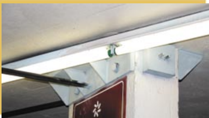
Anchoring at a column
