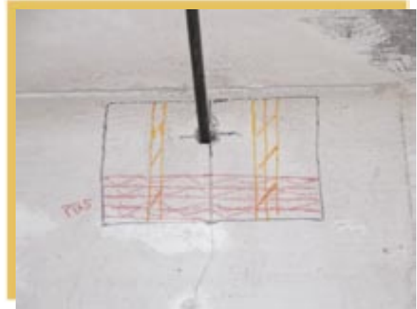
Figure 1: X-ray results showing post-tensioning and stirrups
