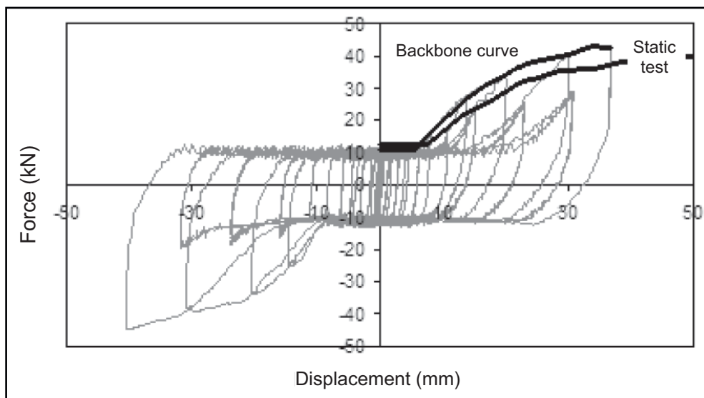
Figure 3: Hysteresis diagram from a fully-reversed quasi-static test of a sill log on a floor diaphragm (from Scott et al. 2005a)
