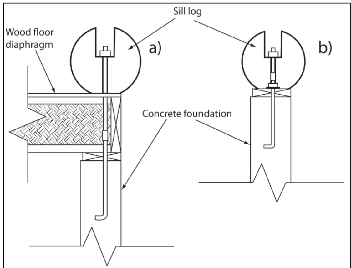
Figure 2: Typical foundation details for log buildings; (a) sill log on floor diaphragm, (b) sill log on concrete foundation wall (from Scott et al. 2005a)
