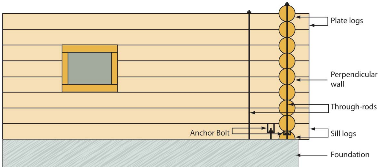
Figure 1: Log wall including a window opening and an inter-wall connection on a rigid foundation (from Scott et al. 2005a)
