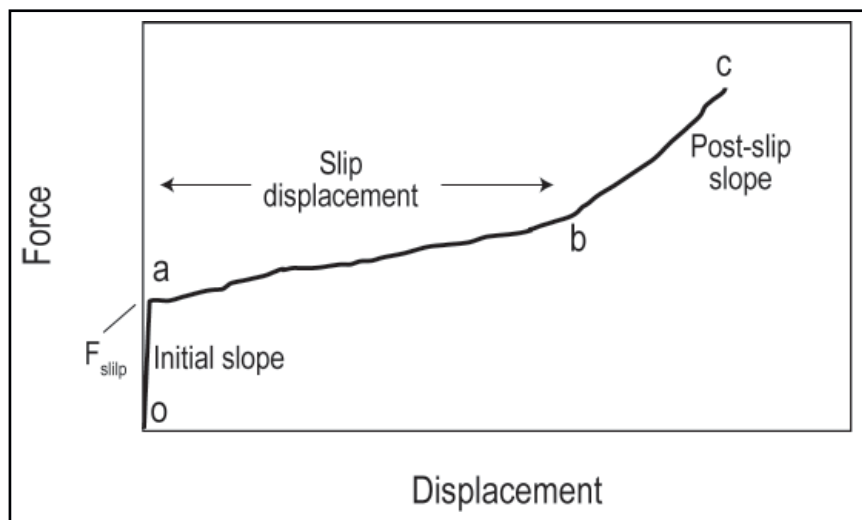
Figure 4: Basic force-displacement curve for a log shear wall with through-rods (Scott et al. 2005b)
