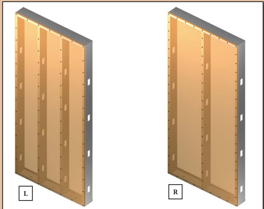
Typical 4 foot wide sheathing with 16-inch on center studs (L) and 24-inch on center studs (R)
