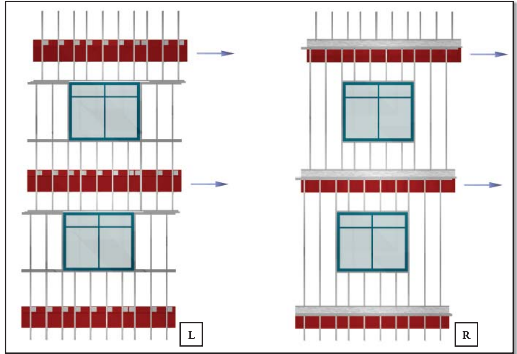
Figure 2: In-plate movement in spandrel framing (L) and floor-to-floor framing (R) with arrows indicating movement direction
