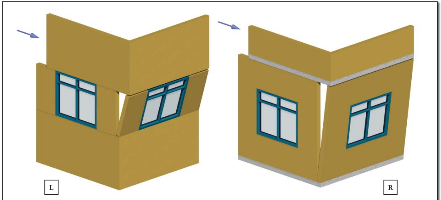
Figure 4: Intersection of walls with spandrel framing (L) and floor-to-floor framing (R) with arrows indicating movement direction
