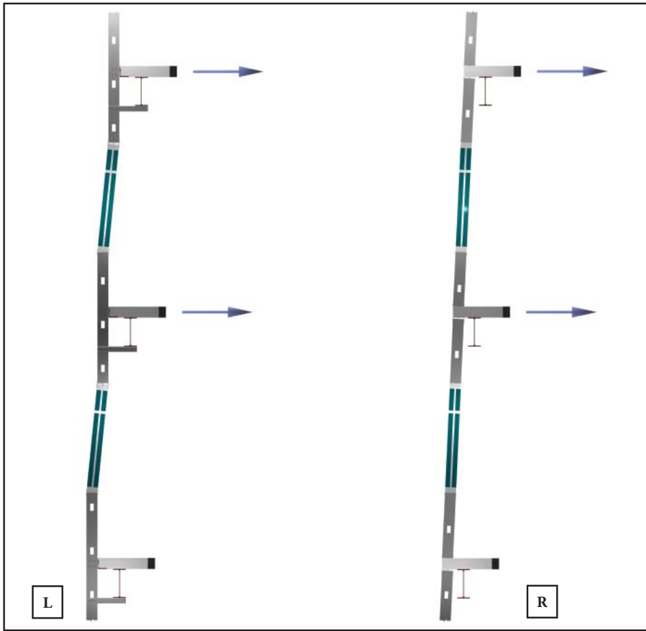
Figure 3: Out-of-plane movement in spandrel framing (L) and floor-to-floor framing (R) with arrows indicating movement direction
