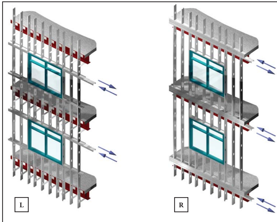
Figure 1: Typical spandrel framing (L) and floor-to-floor framing (R) with arrows indicating potential movement at joint location
