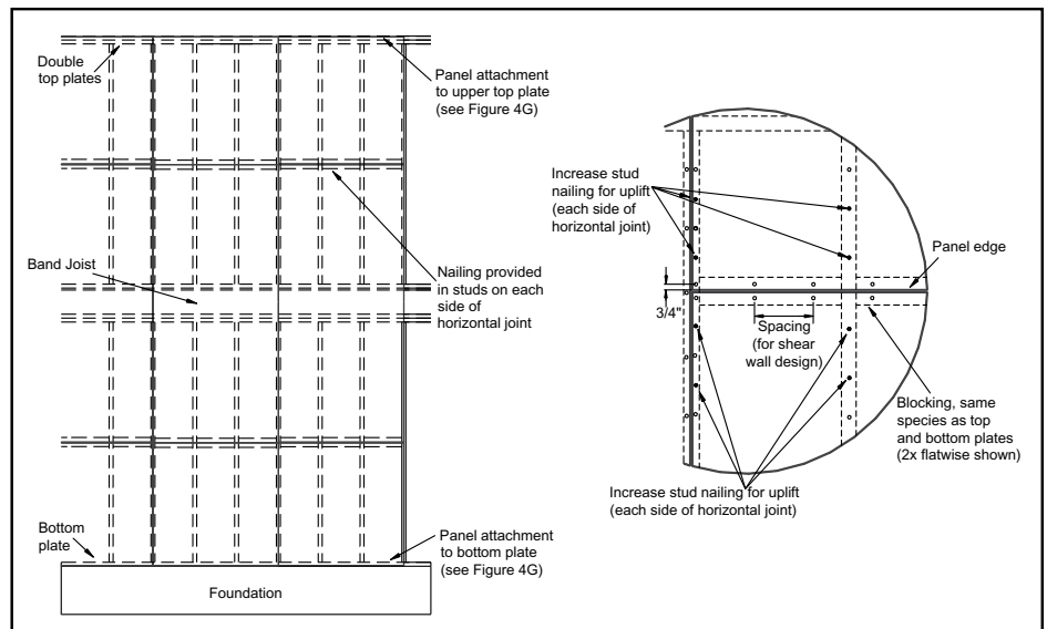
Figure 5b: AWC's Special Design Provision for Wind and Seismic (SDPWS) , 2008 Figure 4I.
