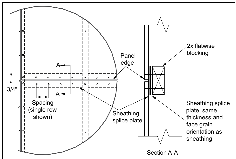
Figure 5c: AWC's Special Design Provision for Wind and Seismic (SDPWS) , 2008 Figure 4J.
