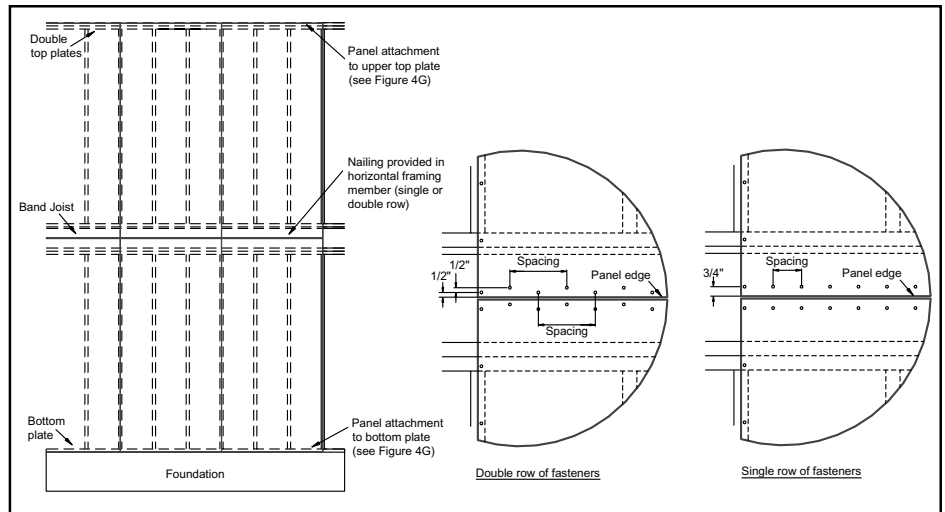
Figure 5a: AWC's Special Design Provision for Wind and Seismic (SDPWS) , 2008 Figure 4H.
