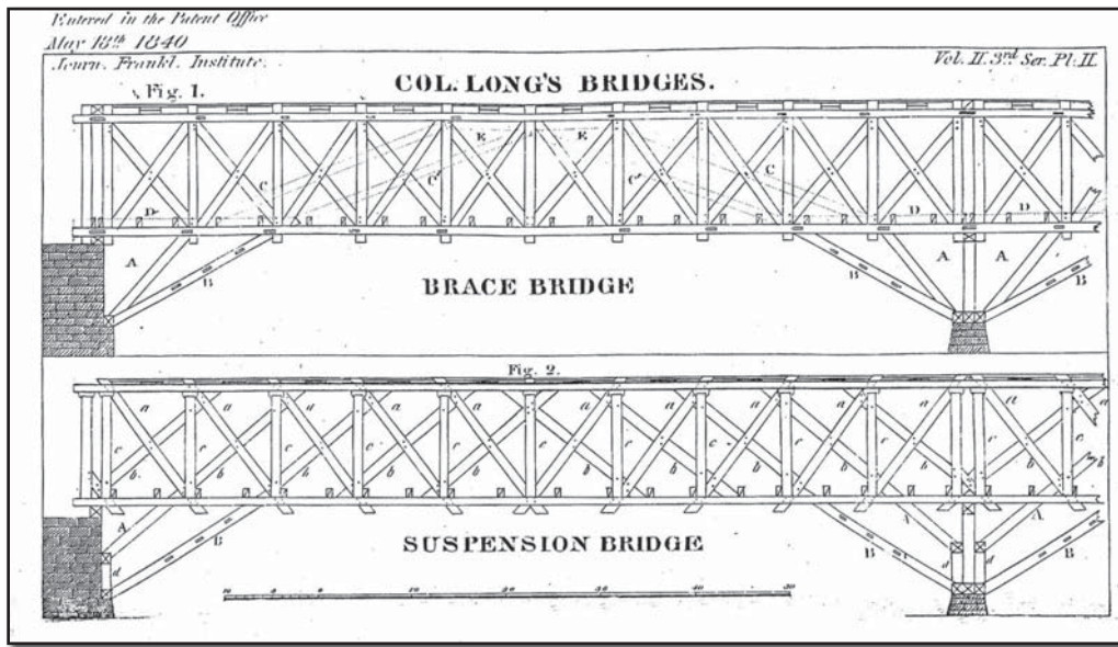
Figure A: Long's Brace and Suspension Bridge Patent #1.397 and 1.398 - November 7, 1839
