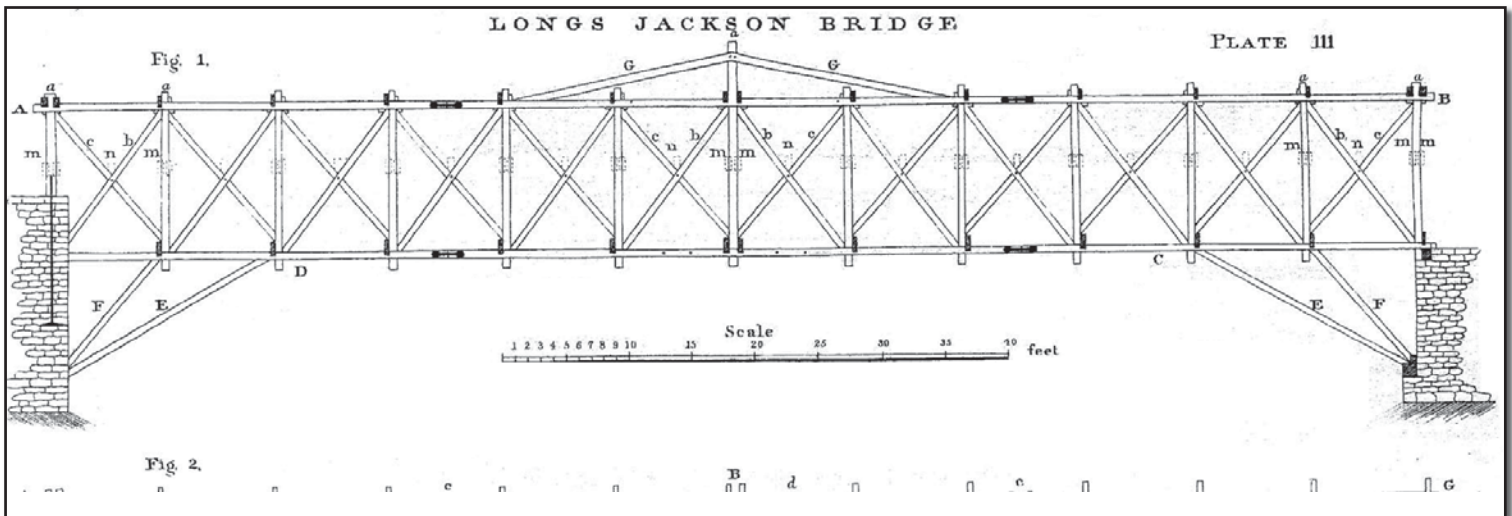
Long's Jackson Bridge 1830
