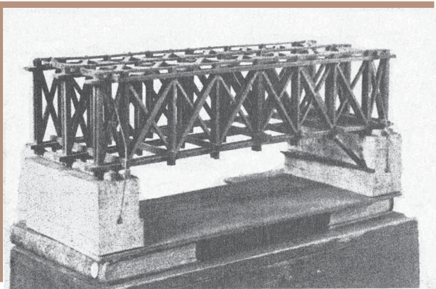
Model of Long's 1830 Patent Jackson Bridge as used by his agents
