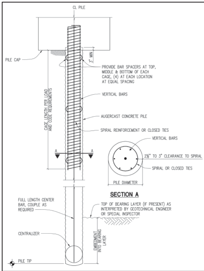
Figure 4: Typical augercast pile detail
