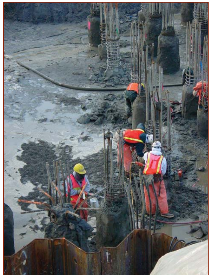
Figure 3: Grout being chipped from the cage
