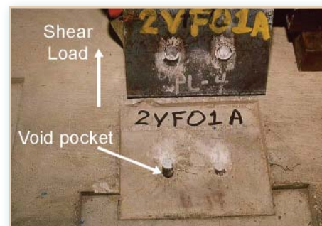
Figure 1: Typical steel failure of a headed-stud connection loaded in shear
