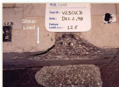
Figure 3: Example of a front edge concrete breakout when the shear force is applied perpendicular (normal) to the edge
