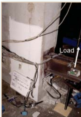
Figure 12: Photograph of combined tension and shear failure on an embedded column corbel plate
