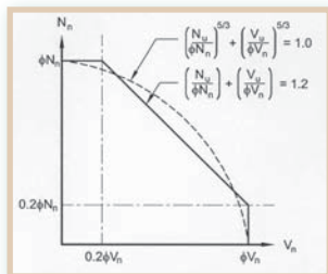
Figure 13: Combined tension and shear relationships permitted by ACI 318-05 Appendix D (plot from PCI Design Handbook [2004])
