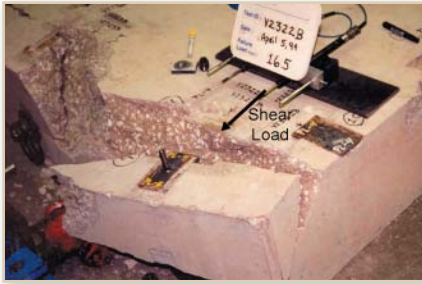
Figure 5: Corner concrete breakout when the shear force is applied perpendicular (normal) to the front edge
