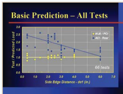
Figure 8: Side-edge breakout comparison of the proposed WJE / PCI equation in the 6th Edition, PCI Design Handbook [PCI 2004] with the present ACI 318-05 Appendix D method
