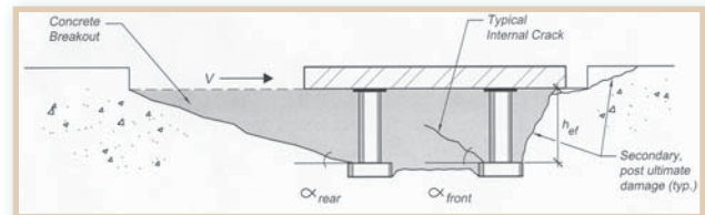
Figure 10: Sketch of a concrete pryout failure (courtesy of PCI Journal)
