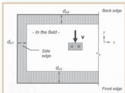
Figure 2: Definitions of edge conditions associated with shear-loaded anchorage groups
