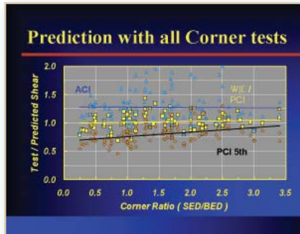
Figure 6: Corner breakout comparison of the proposed WJE / PCI equation in the 6th Edition, PCI Design Handbook [PCI 2004] with the present ACI 318-05 Appendix D and 5th Edition, PCI Design Handbook [PCI 1999]
