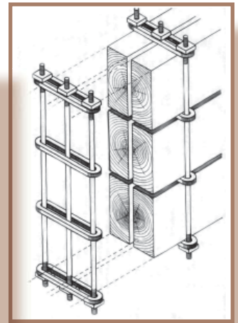
Arch members with spacers
