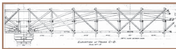
Harper's Ferry B & O Truss by Latrobe/Wernwag
