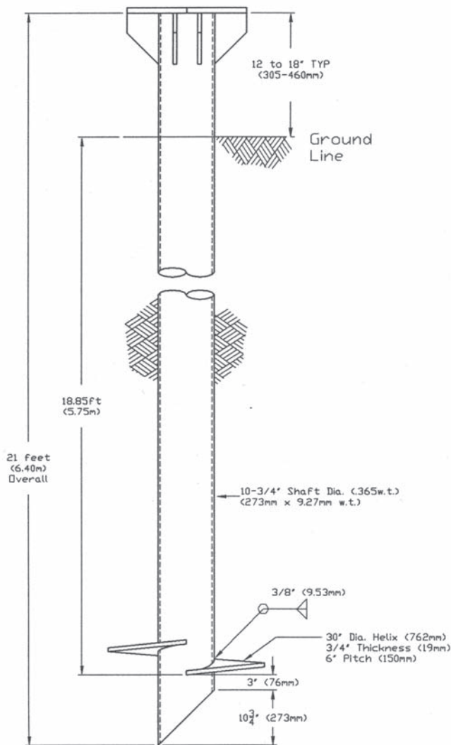
Figure 7: Compression and Tension Screw Piles
