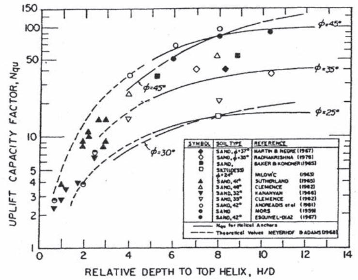
Figure 6: Uplift Capacity Factor, N_{qu} , vs. Embedment Ratio, H/D Ratio for Helical Anchors in Sand
