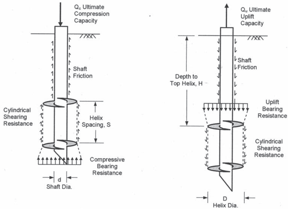
Figure 3: Screw Pile in Compression and Tension Loading
