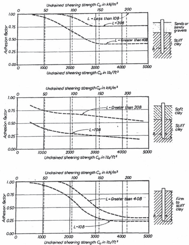
Figure 4: Design Curves for Adhesion Factors for Piles Driven into Clay Soils
