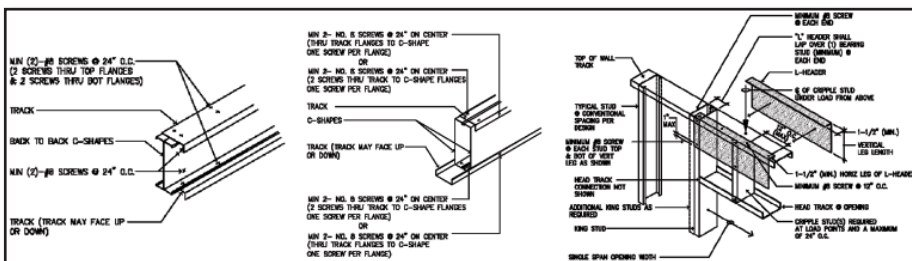
Figure 2 Back-to-Back, Box and L-Header Assemblies
